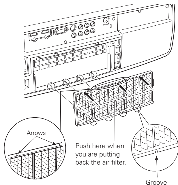
When putting back the air filter, make sure that the arrows on the filter are facing towards the projector.
